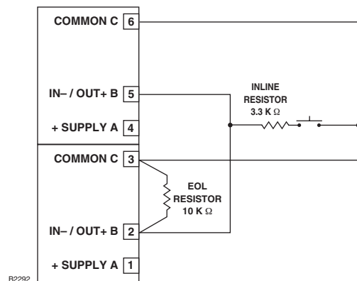
Figure 7—Supervised Input Configuration (Opens and Shorts) – Class A, Style E
