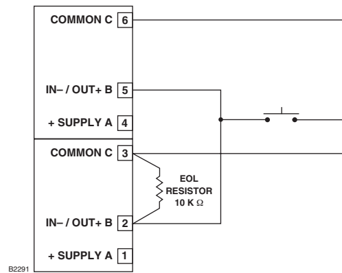
Figure 5—Supervised Input Configuration – Class A, Style D
