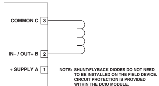
Figure 10—Unsupervised Output Configuration
