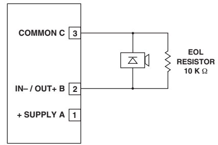
Figure 11—Supervised Output Configuration (Notification)— Class B, Style Y
