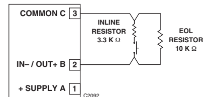
Figure 6—Supervised Input Configuration (Opens and Shorts) – Class B, Style C
