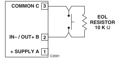
Figure 4—Supervised Input Configuration – Class B, Style B
