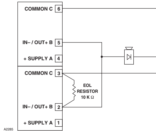
Figure 12—Supervised Output Configuration (Notification)— Class A, Style Z
